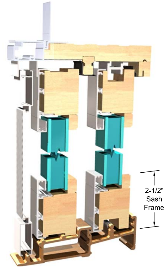
Head/Sill Section Scale: 1/4"=1"
