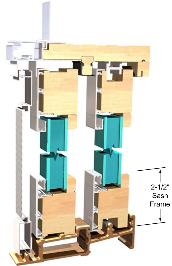
Head/Sill Section Scale: 1/4"=1"
