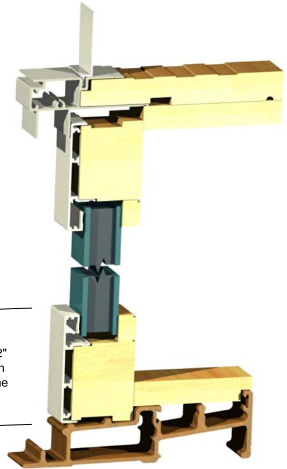
Head/Sill Section
