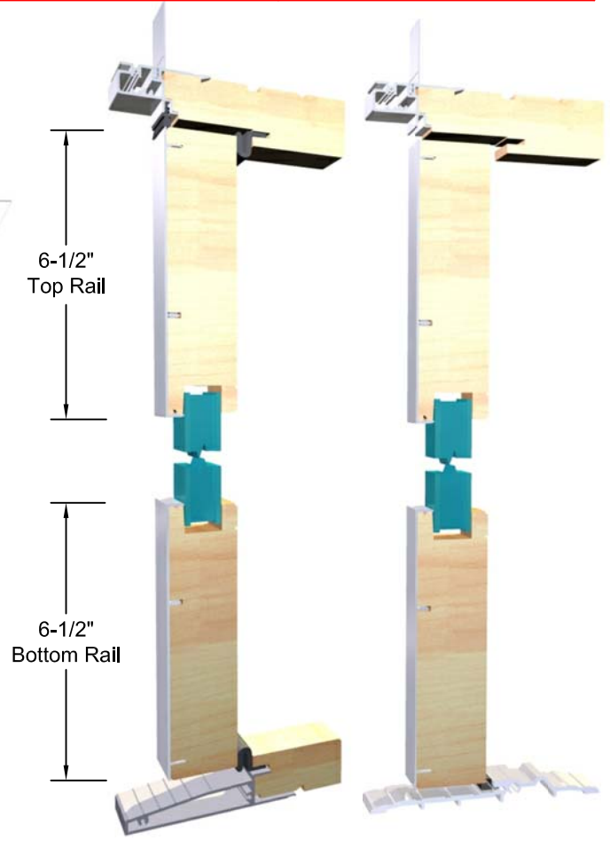
Head/Sill Section Scale: 1/4"=1"
